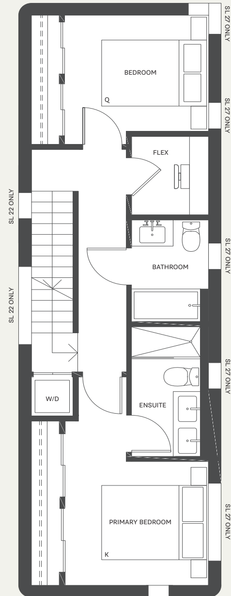
SECOND LEVEL
