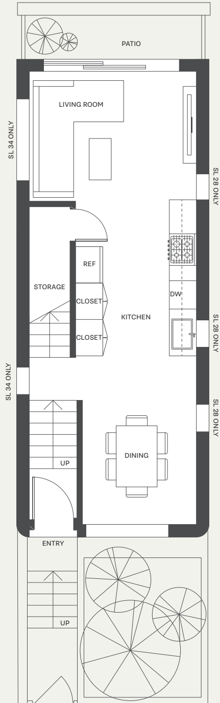
MAIN LEVEL
