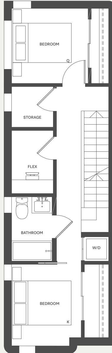
SECOND LEVEL
